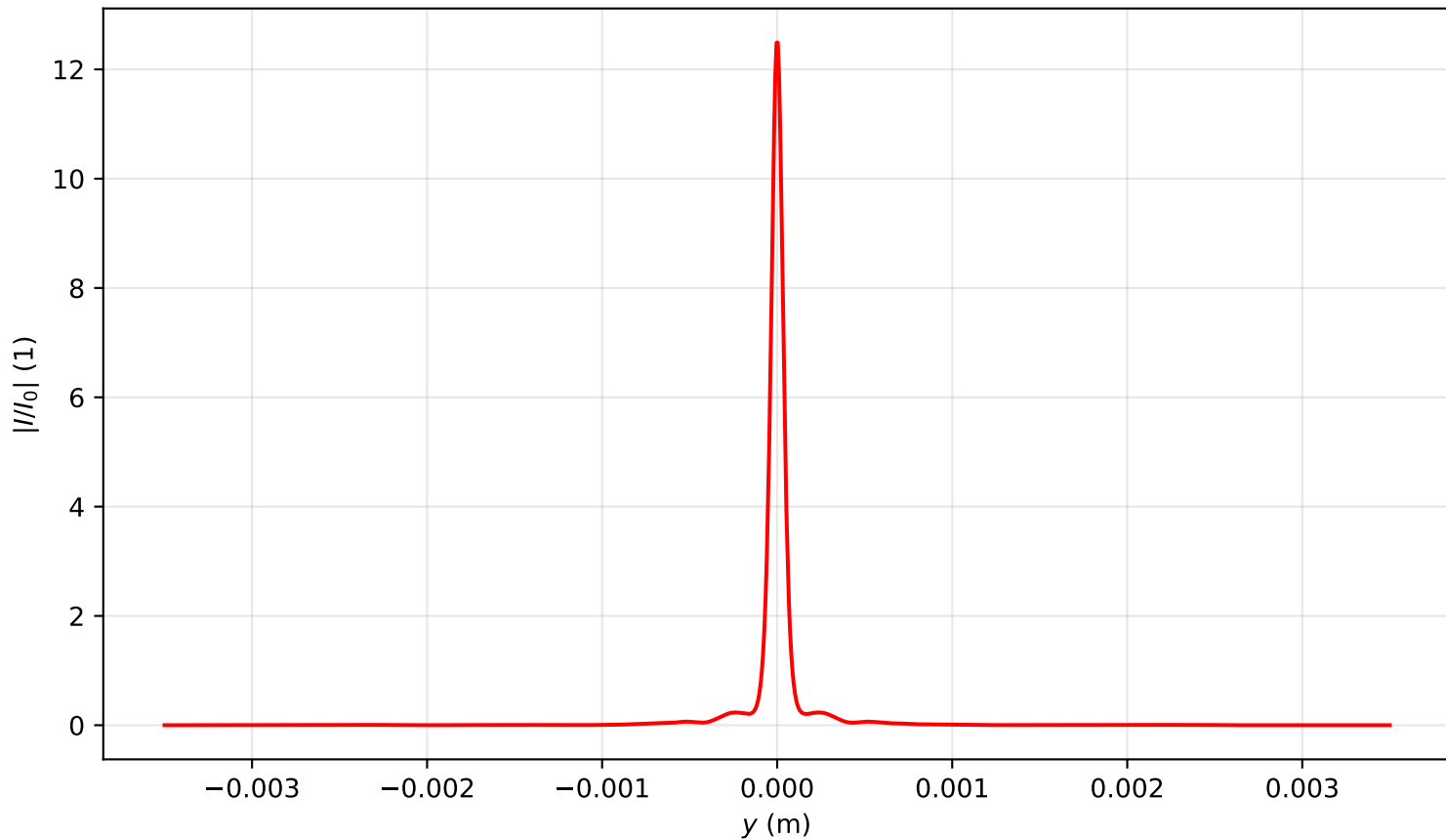
Intensity profile I(x=0, y, z=1.274)/I_0 , P_{in}=4.0P_{cr} , artificial time
